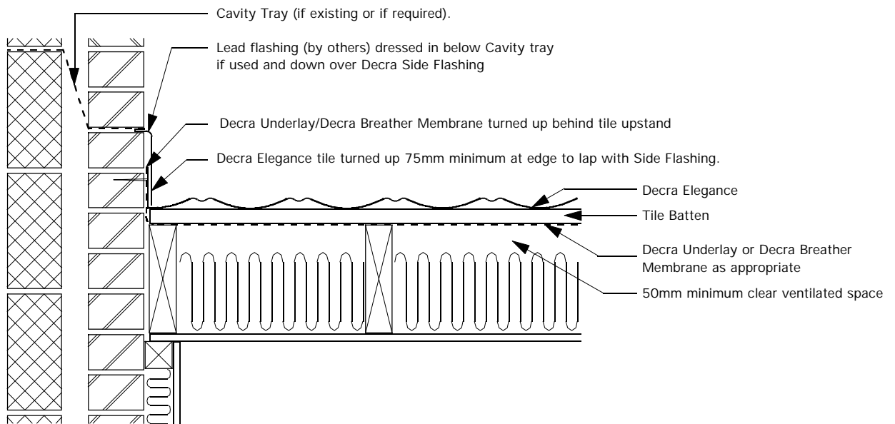
Abutment Detail Without Side Flashing
