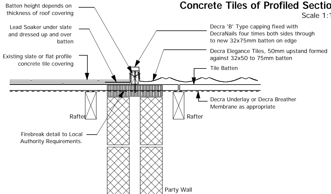
Detail of Decra abutting Slate or flat profile Concrete Tile
